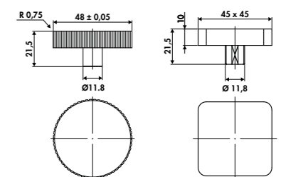
AVCCANNELE / AVCCARREE
