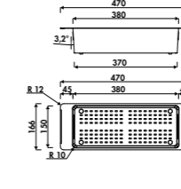
COLANDER / AEPANCOL
