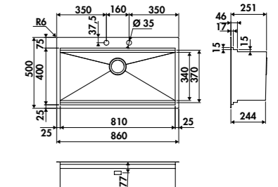
LAB / EV36
